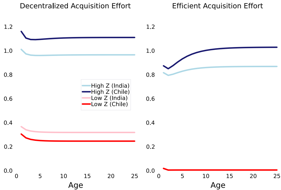
Figure 14: Efficient Supplier Acquisition: Chile vs. India
