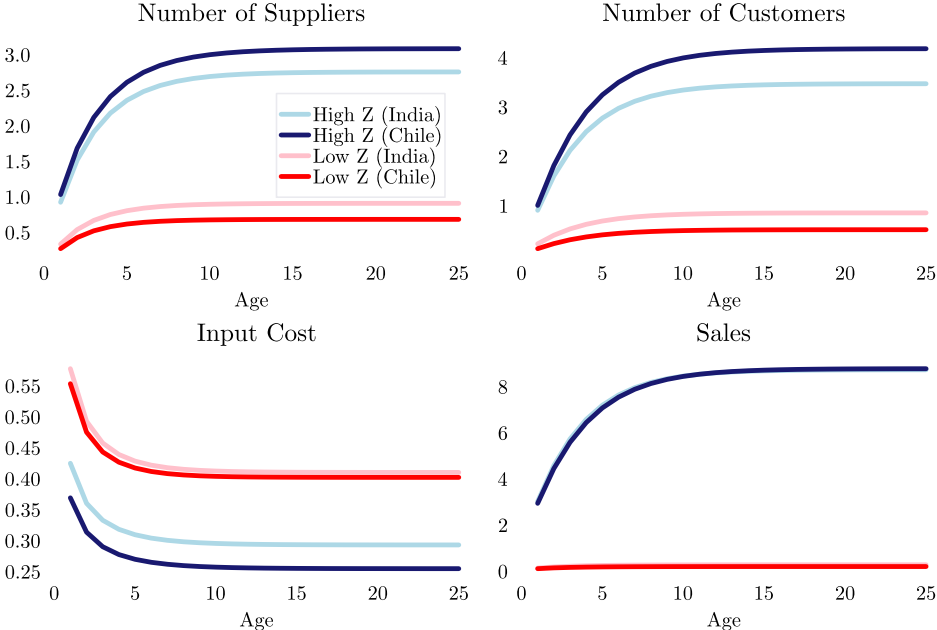
Figure 12: Lifecycle Trajectories of Chilean Firms
