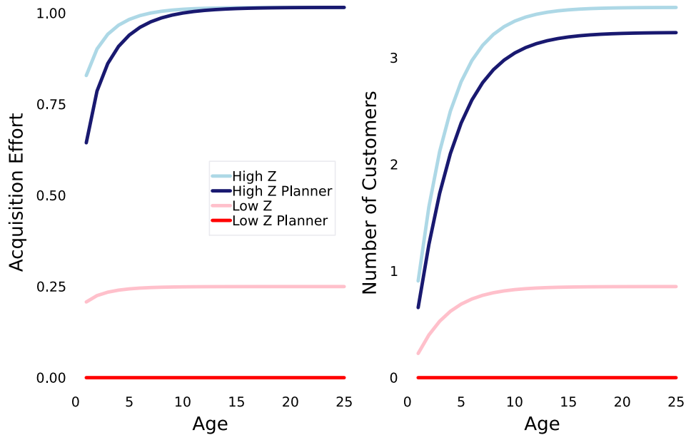
Figure 9: Efficient Customer Acquisition
