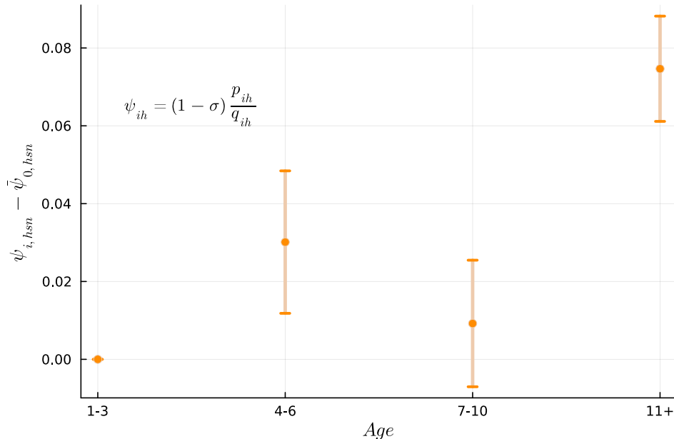
Figure 5: Input Share Supplier Effect \psi_{i,hsn}
