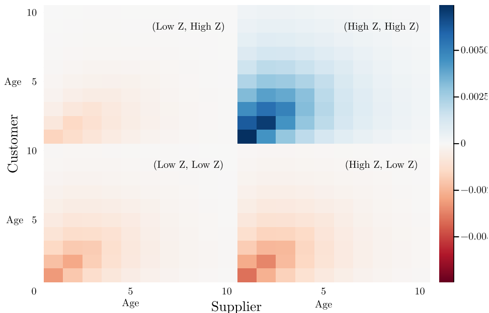
Figure 13: Production Network of Chile vs. India
