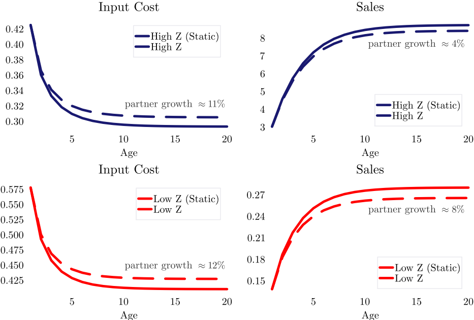
Figure 7: Dynamics Contribution of Trading Partners
