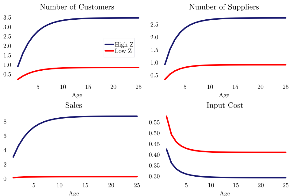
Figure 6: Model Output
